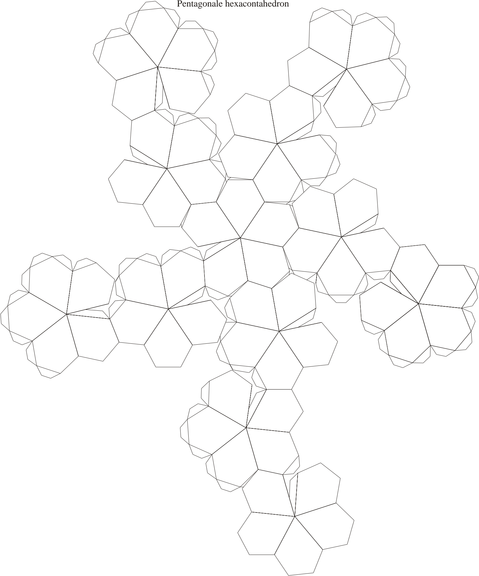
Pentagonale hexacontahedron
