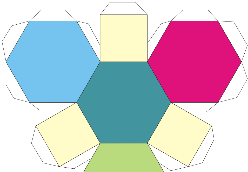
Truncated Octahedron
