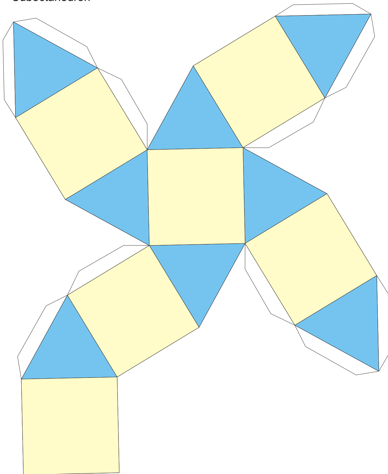
Cuboctahedron
