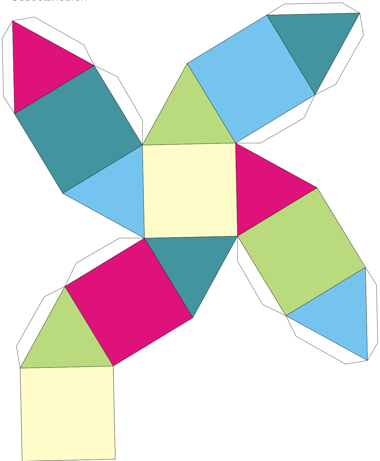
Cuboctahedron
